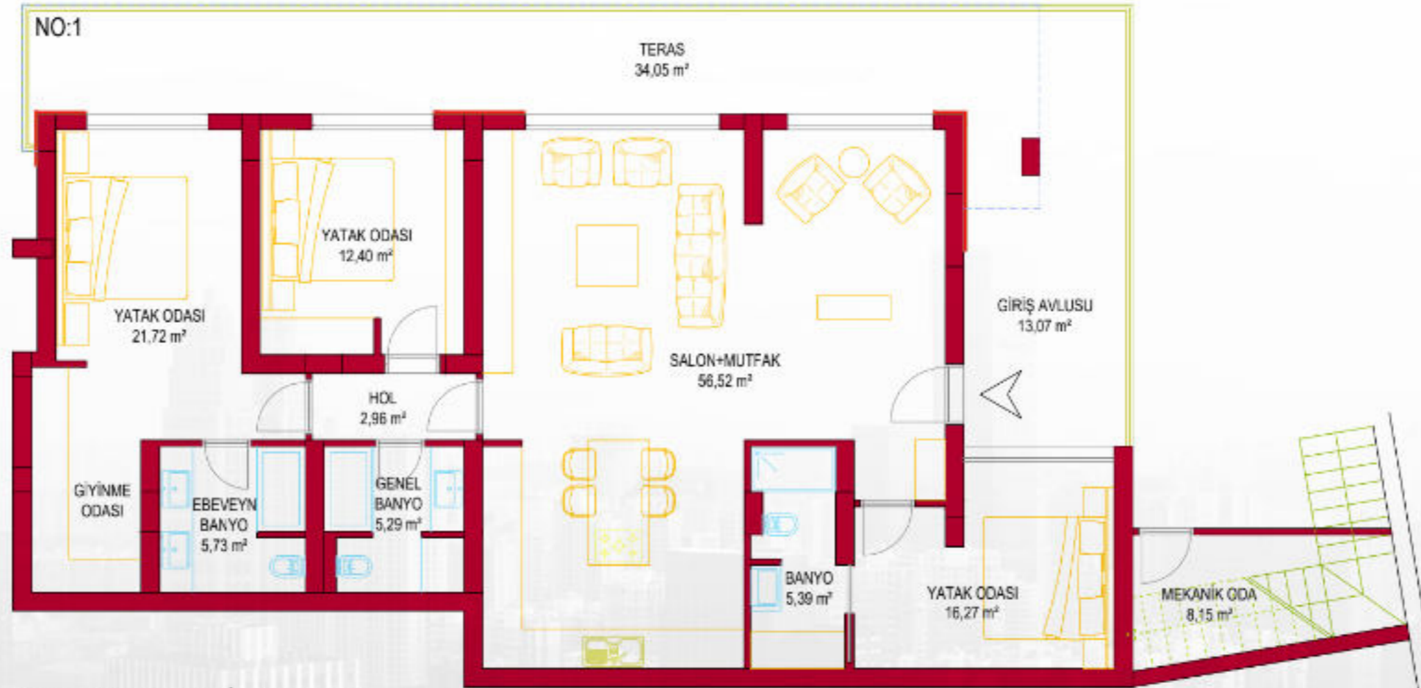
3+1 CR 31 BLOK ZEMİN KAT PLANI
